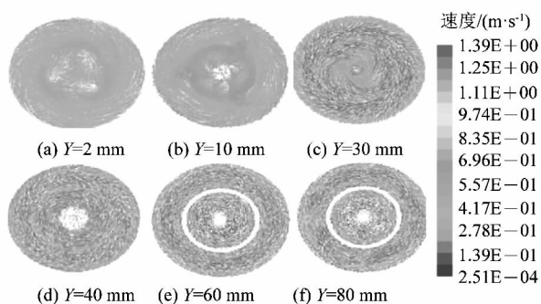
图 13 Y轴各截面速度矢量图 Figure 13 Velocity vector graph of Y axis section
